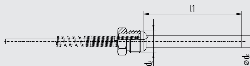
SF91/SV20, male nut with sealing cone
