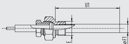
SV20 with thermowell SH16
