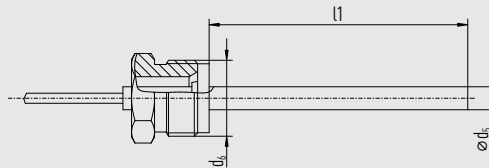
BF2, rotatable threaded connection
