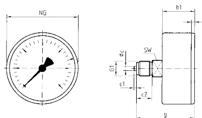
NG 40/50/63 – centre back connection
