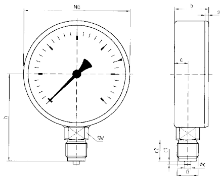
NG 100 – bottom connection
