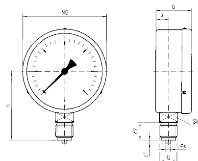
Bottom connection
