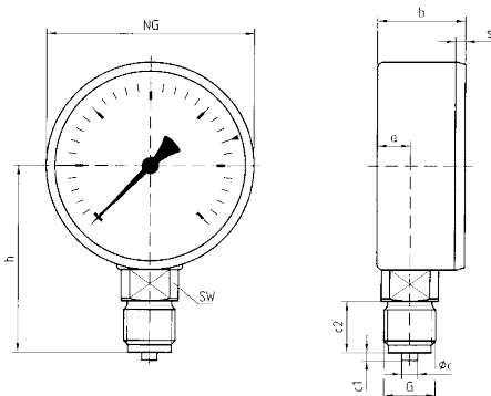
NG 100 – bottom connection
