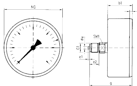
NG 100 – centre back connection
