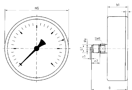
NG 100 – centre back connection
