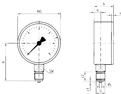
NG 80 – bottom connection
