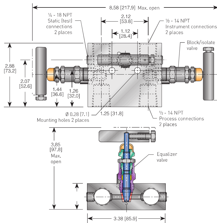
M1 SOFT SEAT DIMENSIONS, INCHES [mm]
